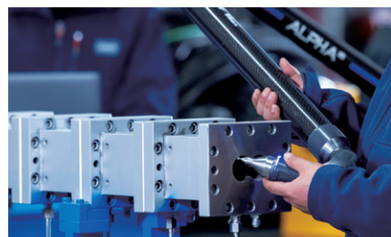
Three-coordinate measuring machine measures overall coaxiality
